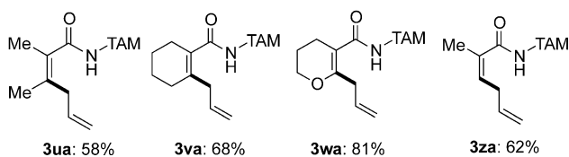
Scheme 1. Iron-catalyzed C–H allylation with allyl chloride ( 2a ).
